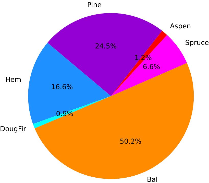
Species Distribution at Time Period 0
